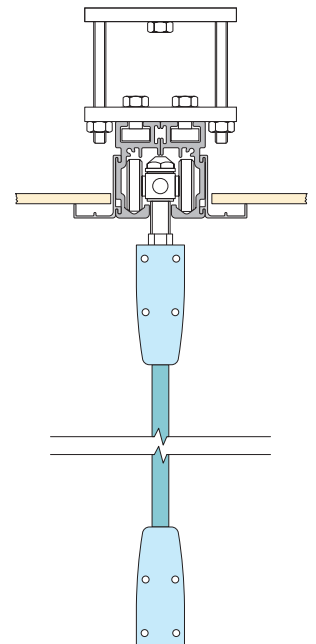
Track Detail
