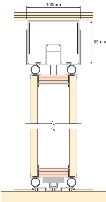
Floor Mounted
