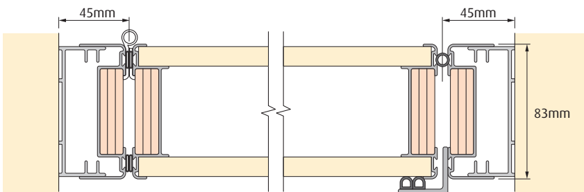
Horizontal Section
