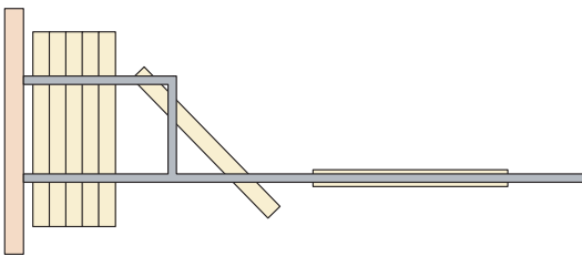
90° Side stack
