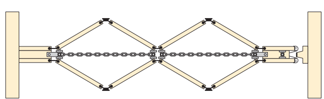
Track detail
