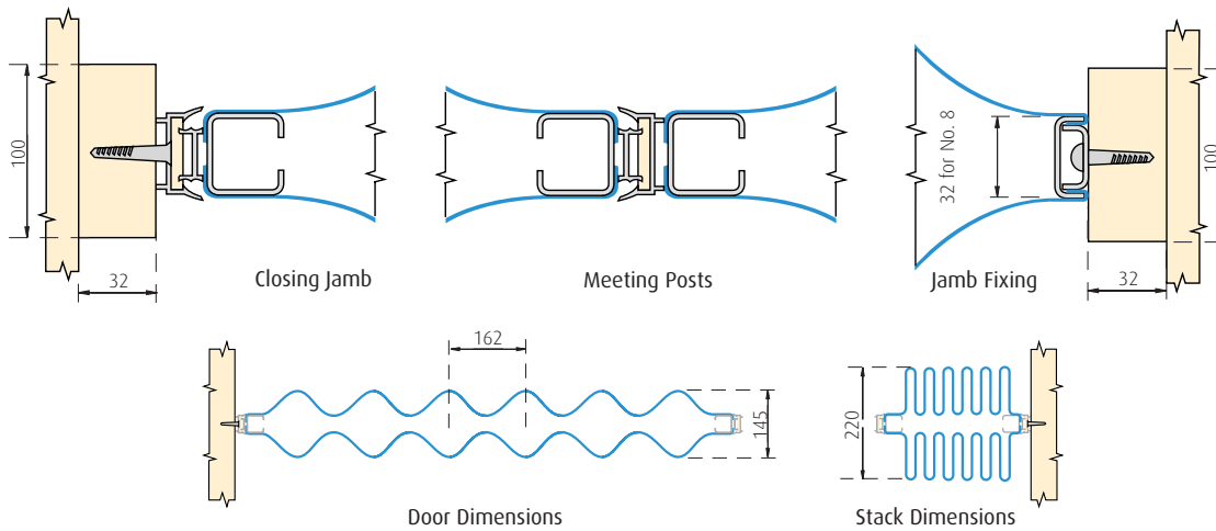
No. 8 Standard Track-Exposed
