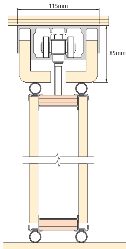
Top Hung
