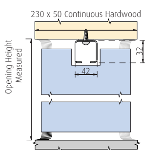
No. 8 Standard Track-Exposed
