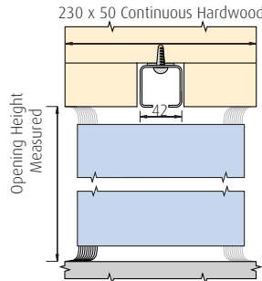
No. 8 Standard Track-Recessed
