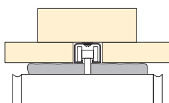
Track with Acoustic seal
